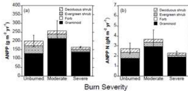
Fig. 39. (a) Above-ground net primary productivity (ANPP) and (b) ANPP Nitrogen for four plant functional types in unburned, moderately burned and severely burned tundra following the Anaktuvuk River fire of 2007 on the North Slope of Alaska (Bret-Harte et al. 2013).
