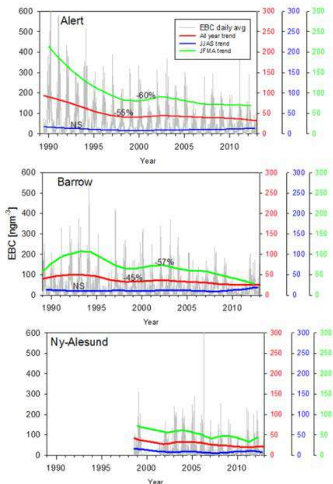
Fig. 16. Daily-average surface equivalent black carbon (EBC) at Alert, Barrow and Ny-Ålesund. Trend lines (green, red, blue) were determined using the LOWESS technique (LOcally WEighted Exponentially Scatterplot Smoothing). The red line includes all EBC data, the green line is the average for January to April (JFMA), and the blue line is the average for June to September (JJAS). The % change in EBC between 1990-1993 and 2009-2012 is given for each trend line for Alert and Barrow. No significant (NS) change occurred in summer at those locations.
