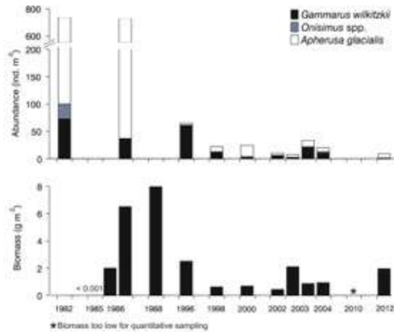
Fig. 26. (a, top) Abundance (ind. m^{-2} ) estimates of the most common ice amphipod species, and (b, bottom) estimates of biomass (wet weight, g\ m^{-2} , for all three species combined) between July and September in sea ice north of Svalbard ( >79^{\circ}N ). Abundance and biomass data are not always available for the same years. Data are from Hop and Pavlova (2008), Lønne and Gulliksen (1991a, b) and also include unpublished data from the Norwegian Polar Institute (H. Hop), the UiT- The Arctic University of Norway (B. Gulliksen) and the University Centre in Svalbard (O. J. Lønne, J. Berge).
