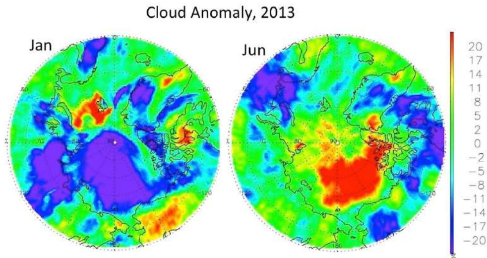
Fig. 6. Cloud cover anomalies (%) in (a, left) January and (b, right) June 2013. The anomalies are calculated relative to the long-term (2002-2011) mean for each month from observations by the Moderate Resolution Imaging Spectroradiometer (MODIS) on the Aqua satellite. Data are from the MODIS L1 and Atmosphere Archive and Distribution System (LAADS) of the Goddard Space Flight Center.
