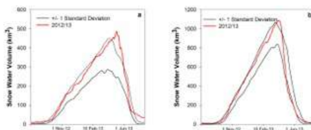
Fig. 49. Daily 2012-13 time series (red) of Arctic snow water volume for (a, left) North America and (b, right) Eurasia derived from the CMC snow depth analysis. The solid black lines show the +/- 1 standard deviation range about the mean SWE over 1998-99 to 2011-12 snow seasons. Note the different y-axis range of each graph.
