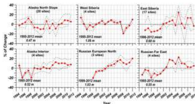
Fig. 65. Active-layer change in six different Arctic regions according to the Circumpolar Active Layer Monitoring (CALM) program ( http://www.gwu.edu/~calm/ ). The data are presented as annual percentage deviations from the mean value for the period of observations (indicated in each graph). The number of CALM sites within each region varies and is indicated in each graph. Thaw depth observations to the end of the thawing season were used. Availability of at least ten years of continuous thaw depth observations through the 2012 thawing season was the only criterion for site selection. Solid red lines show mean values for the regions. Dashed grey lines represent maximum and minimum values for the region.
