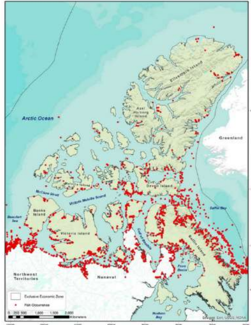
Fig. 32. Fish occurrence records within the Canadian Arctic Archipelago. Inland points represent occurrences of anadromous species adjacent to marine locations. Point locations in deeper areas north of the Archipelago represent pelagic species (e.g., polar cod) captured through or in sea ice.
