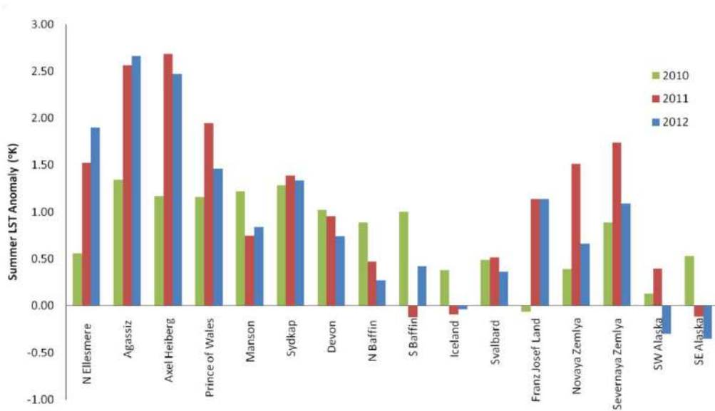
Fig. 53. Comparison of summer mean land-surface temperature (LST) anomalies (relative to 2000-2010 means) in 2010, 2011 and 2012 for 16 glaciated regions of the Arctic based on the MODIS MOD11A2 LST product (ORNL DAAC 2010). Locations of these regions (A, B, C, ..... P) are identified in Fig. 50.
