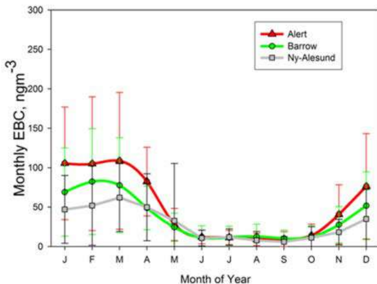
Fig. 18. Seasonal variations in monthly average equivalent black carbon (EBC) at Alert (1989-2012), Barrow (1989-2012) and Ny-Ålesund (1998-2011) show higher EBC values during the winter-spring Arctic haze period. The error bars represent one standard deviation of each mean EBC value.
