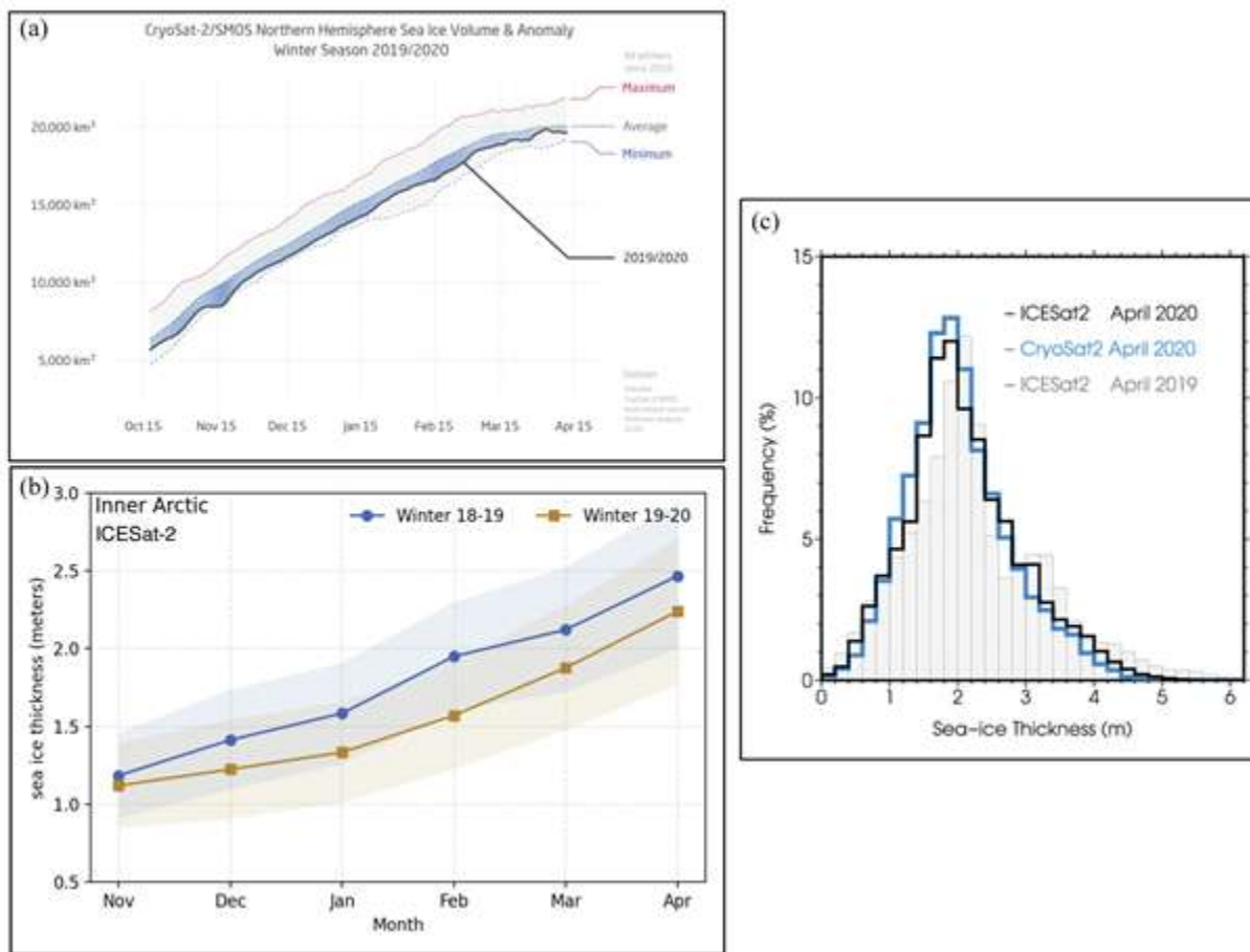
Fig. 4. (a) Time series of Northern Hemisphere sea ice volume from CryoSat-2/SMOS in winter 2019/20, spanning 15 October 2019 to 15 April 2020 (black line). The 10-year climatology range (gray shading) for winter 2010/11 through winter 2019/20 bounded by the daily lowest (Minimum, blue dashed line), highest (Maximum, red dashed line), and average (gray dot-dashed line) sea ice volume in the climatology. Blue shading represents the amount below average of the 2019/20 volume. (b) Monthly thickness from the gridded ICESat-2 product (snow depth/density from modified Warren et al. (1999) climatology) for November to April of 2018/19 (blue) and 2019/20 (brown). Shading represents the mean thickness uncertainty as described in Petty et al. (2020). (c)
