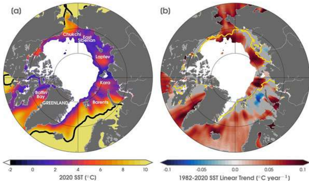
Fig. 1. (a) Mean SST ( ^\circ\text{C} ) in August 2020. White shading is the August 2020 mean sea ice extent, and black contours indicate the 10^\circ\text{C} SST isotherm. (b) Linear SST trend ( ^\circ\text{C yr}^{-1} ) for August of each year from 1982 to 2020. The trend is only shown for values that are statistically significant at the 95% confidence interval; the region is grey otherwise. The yellow line indicates the median ice edge for August 1982-2010. White shading is the August 2020 mean sea ice extent. (Sources: SST data are from the NOAA OISSTv2; sea ice extent and ice-edge data are from NOAA/NSIDC Climate Data Record of Passive Microwave Sea Ice Concentration, Version 3; Peng et al. 2013; Meier et al. 2017.)
