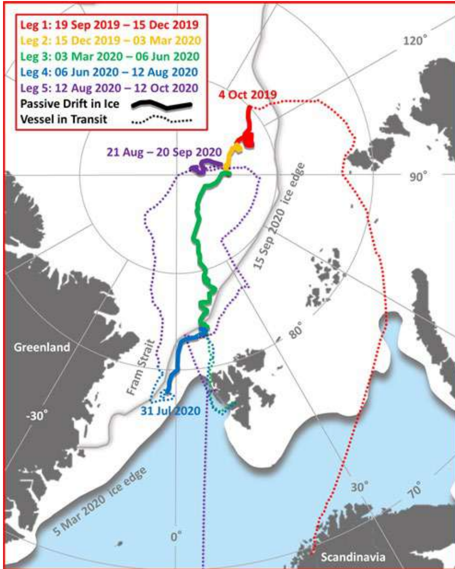
Fig. 2. The MOSAiC Expedition route, including the passive drift of the MOSAiC ice camp (solid) with dates of drift annotated, and in transit movements of Polarstern (dashed) delineated by legs (colors).
