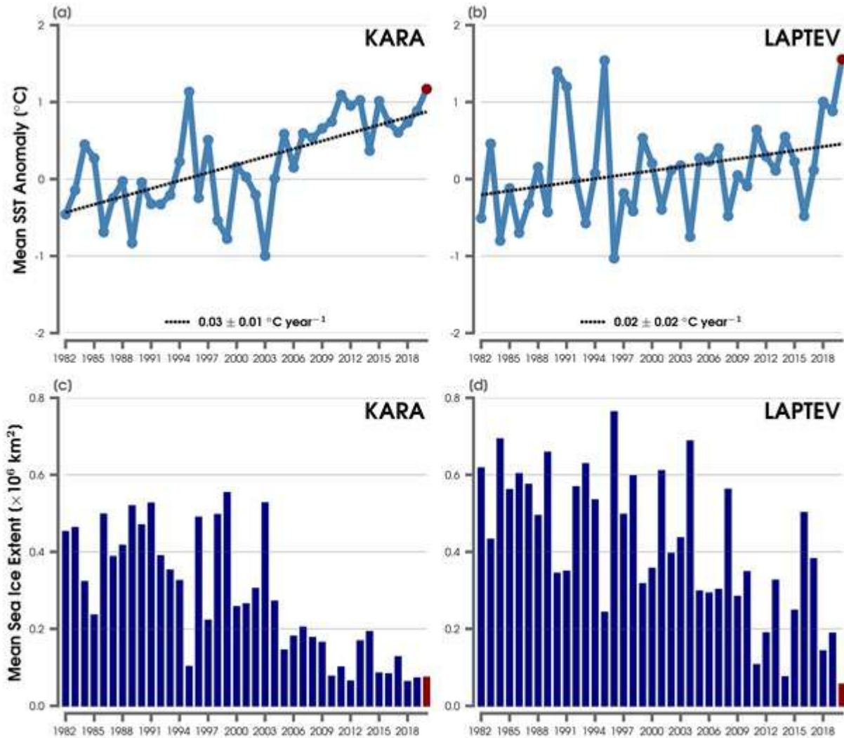
Fig. 3. Area-averaged SST anomalies ( ^\circ\text{C} ) for August of each year (1982-2020) relative to the 1982-2010 August mean for (a) the Kara Sea and (b) the Laptev Sea regions shown by blue boxes in Fig. 2. The dotted lines show the linear SST anomaly trends over the period shown, and numbers in the legends indicate the trends in ^\circ\text{C year}^{-1} (with 95% confidence intervals). August sea ice extents calculated over the (c) Kara and (d) Laptev Sea domains. Sea ice extent data are from NSIDC Sea Ice Index, Version 3 (Fetterer et al. 2017) using a regional mask introduced by Meier et al. (2007), available at nsidc.org .
