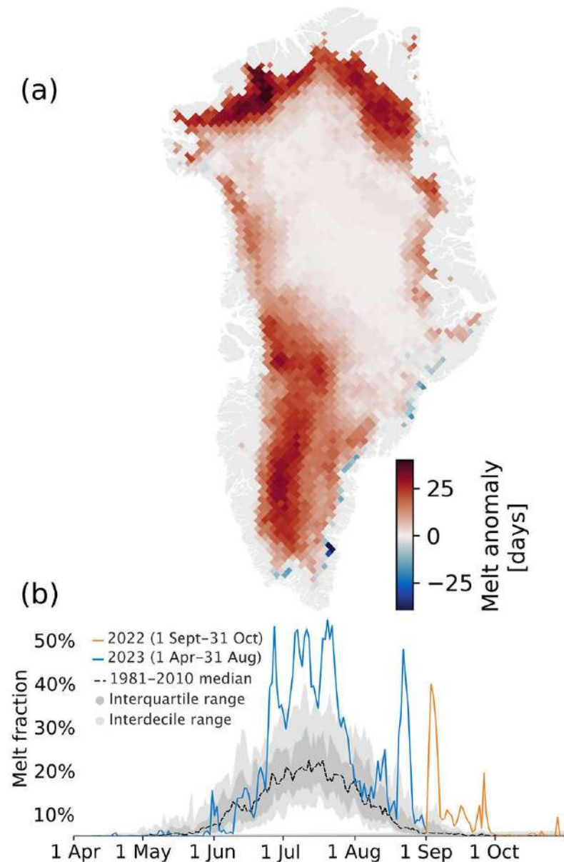
Fig. 2. (a) Number of surface melt days in 2023 from 1 April to 31 August, expressed as an anomaly with respect to the 1991-2020 period from daily Special Sensor Microwave Imager/Sounder (SSMIS) 37 GHz horizontally polarized passive microwave radiometer satellite data (Mote 2007). (b) Surface melt extent as a percentage of the ice sheet area during 2023 (blue) and autumn 2022 (orange) derived from SSMIS.
