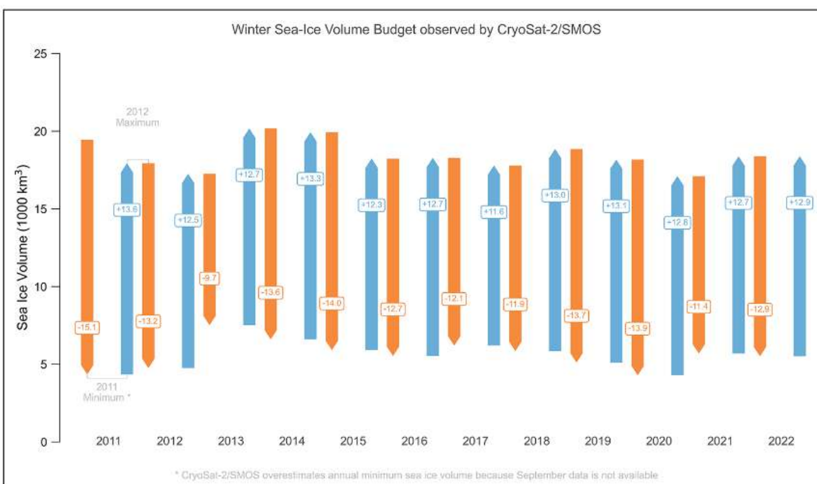
Fig. 5. Annual sea ice volume loss (orange) and gain (blue) between annual maximum and minimum from CryoSat-2/SMOS. Numbers in orange and blue indicate the total volume change (gain or loss) in smaller font with signed values.
