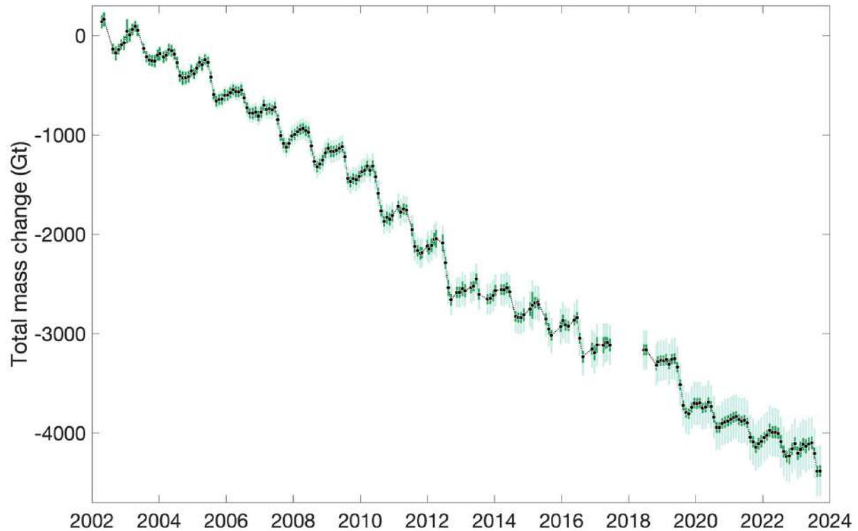
Fig. 1. GRACE-based mass balance. Total mass change, in gigatonnes (Gt), of the GrIS from April 2002 through September 2023 determined from the satellite gravimetry missions GRACE (2002-17) and GRACE-FO (2018-present) (Tapley et al. 2019). Black circles show monthly estimates, with 2-st. dev. uncertainties shown with (light green) and without (dark green) errors due to leakage of external signals (i.e., mass changes near Greenland but not associated with the GrIS). The time series has been scaled by 0.84 to remove the peripheral glaciers and ice caps from the GRACE-based estimates.
